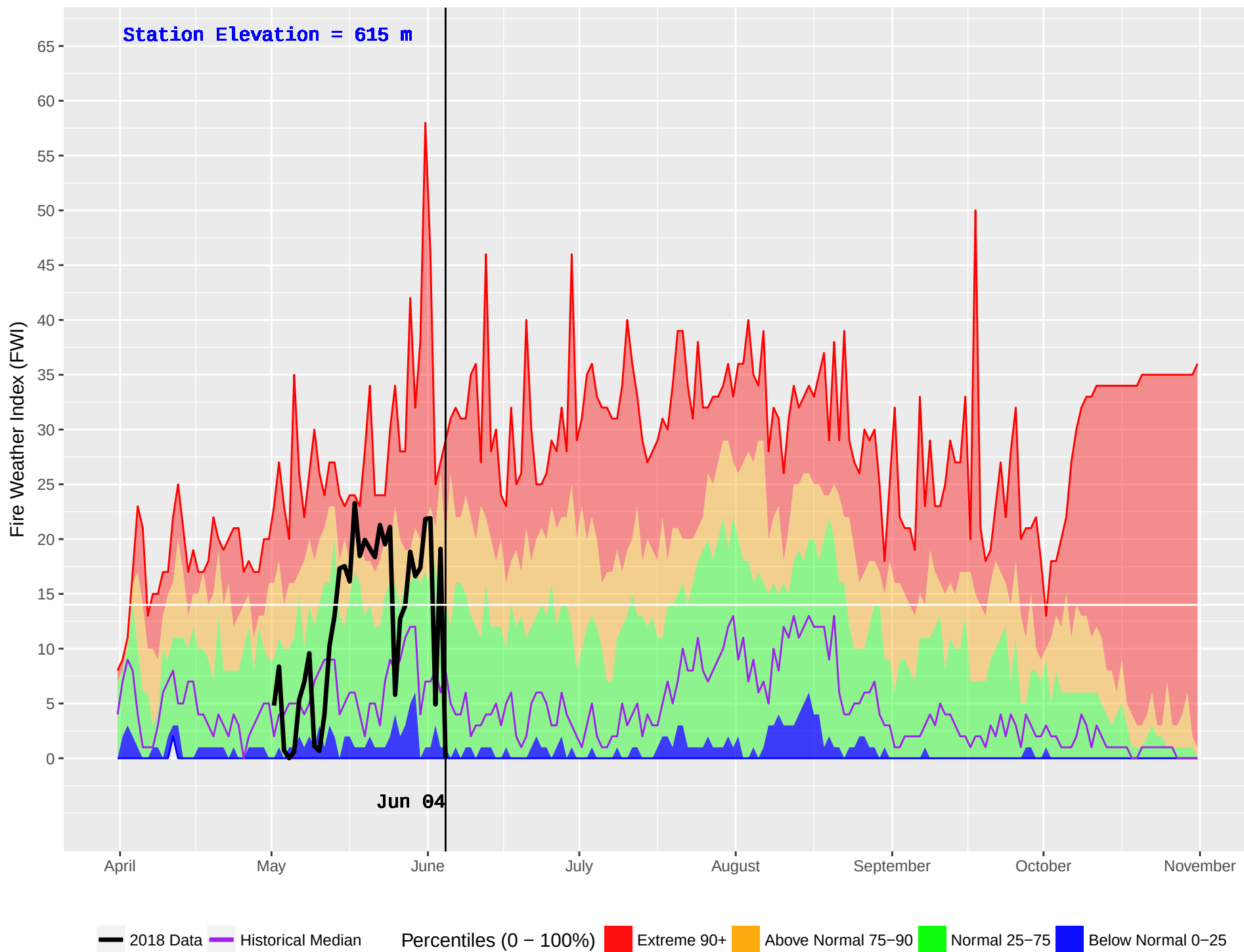
HIXON (187) : Historical (1976–2016) and Current (2018) Noon Fire Weather Index (FWI)
