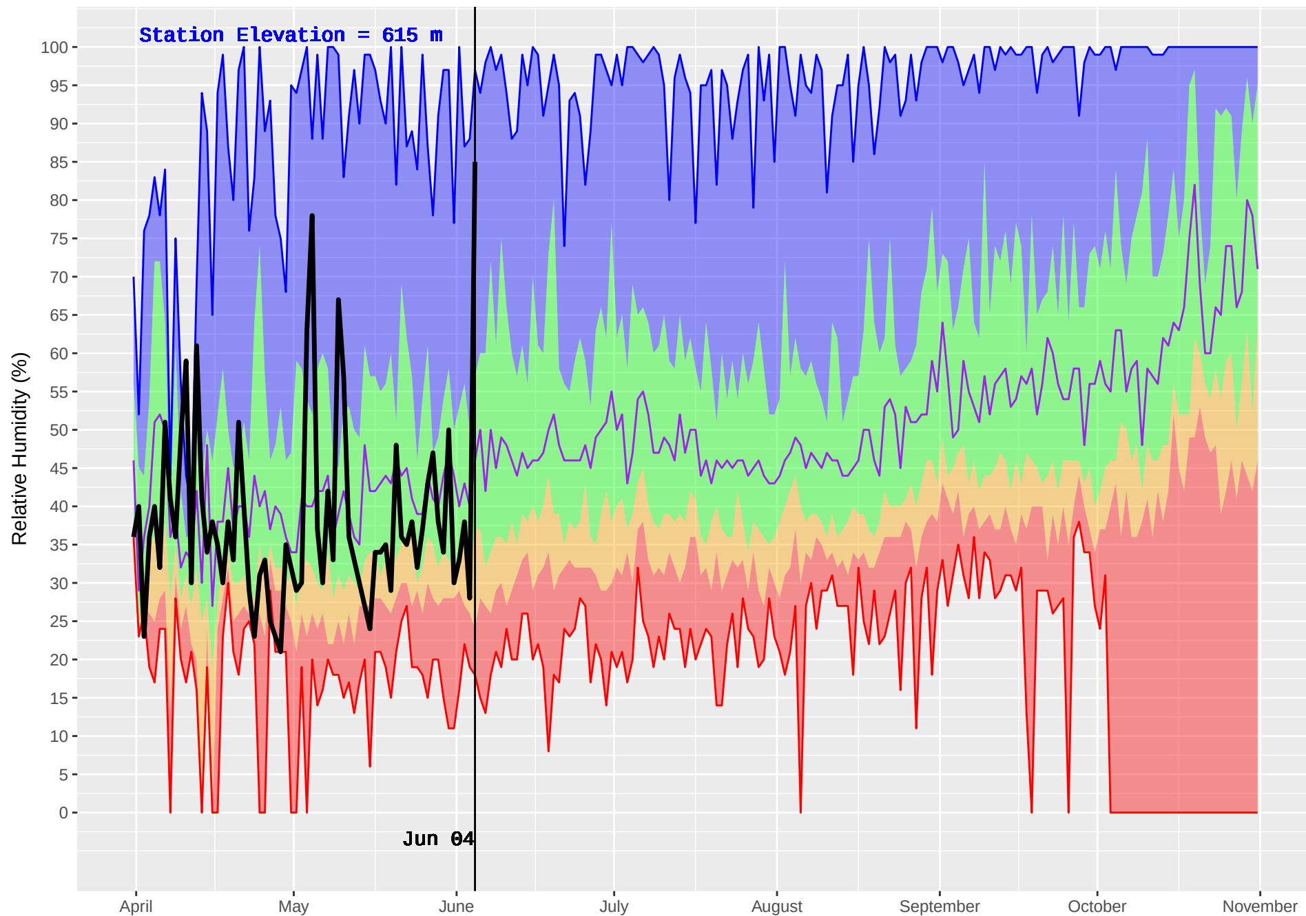
HIXON (187) : Historical (1976–2016) and Current (2018) Noon Relative Humidity
