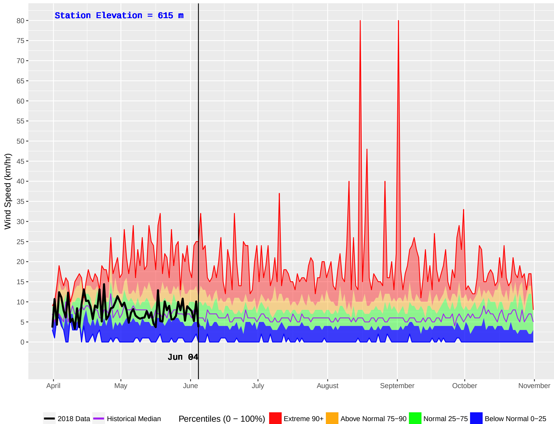
HIXON (187) : Historical (1976–2016) and Current (2018) Noon Wind Speed
