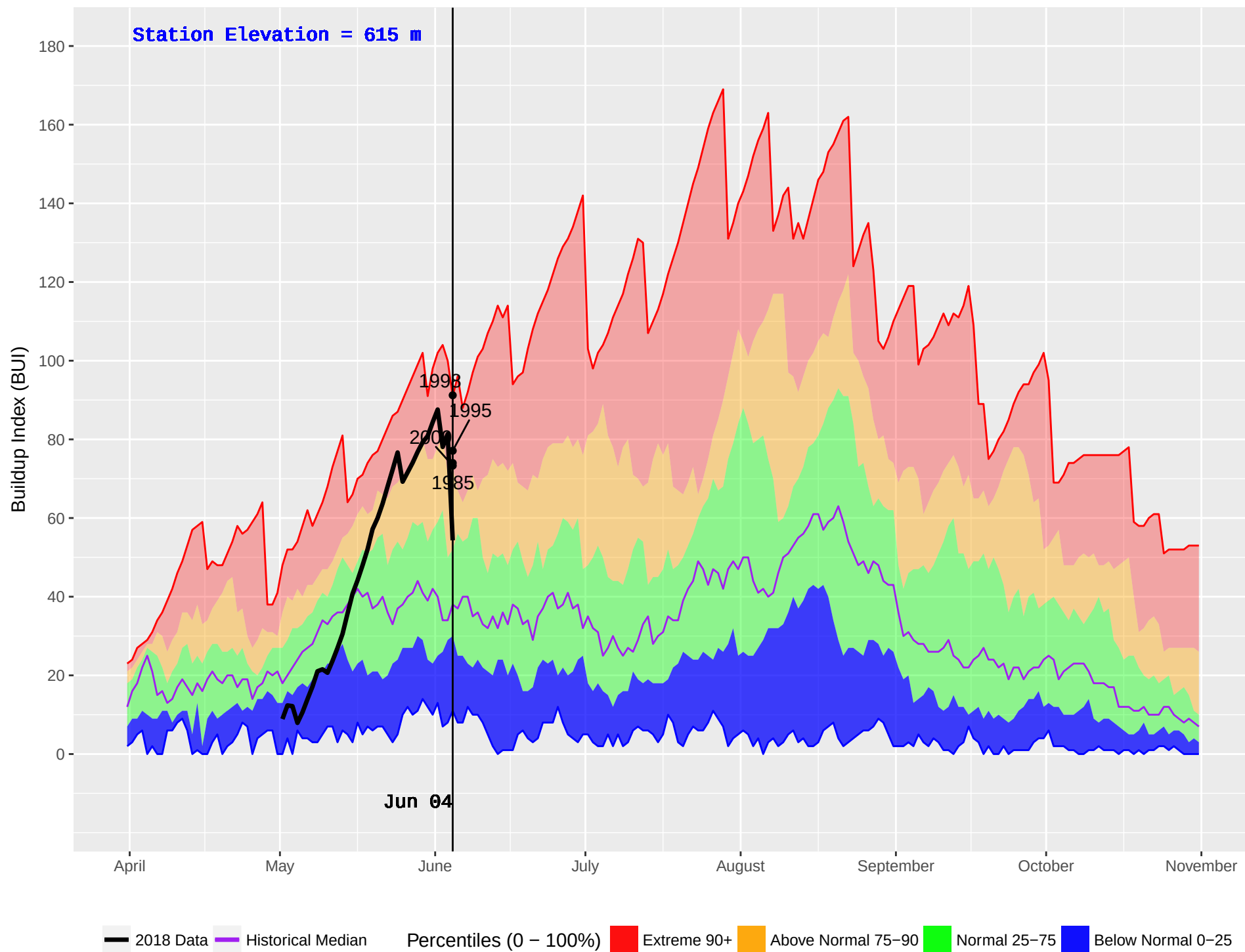
HIXON (187) : Historical (1976–2016) and Current (2018) Noon Buildup Index (BUI)
