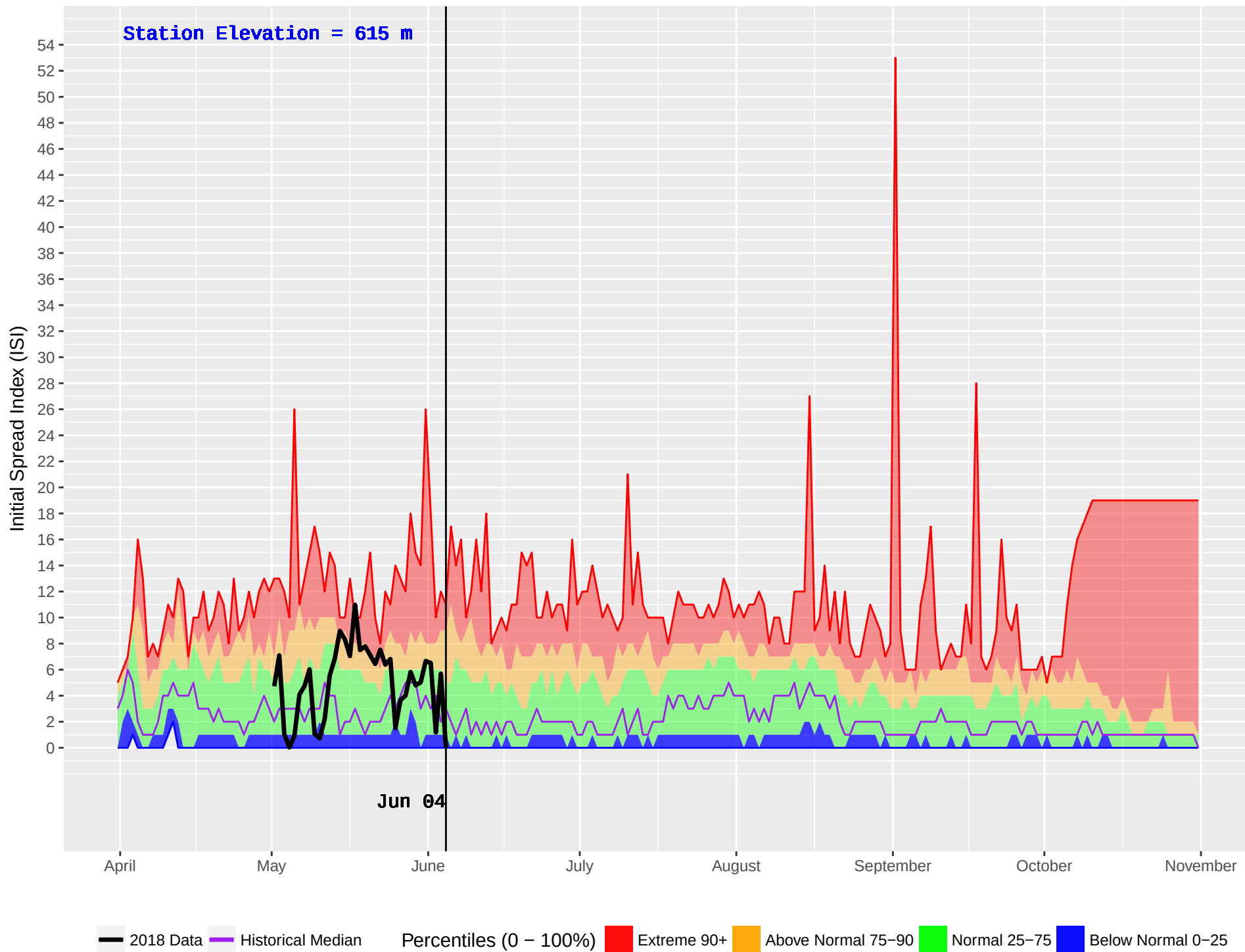
HIXON (187) : Historical (1976–2016) and Current (2018) Noon Initial Spread Index (ISI)
