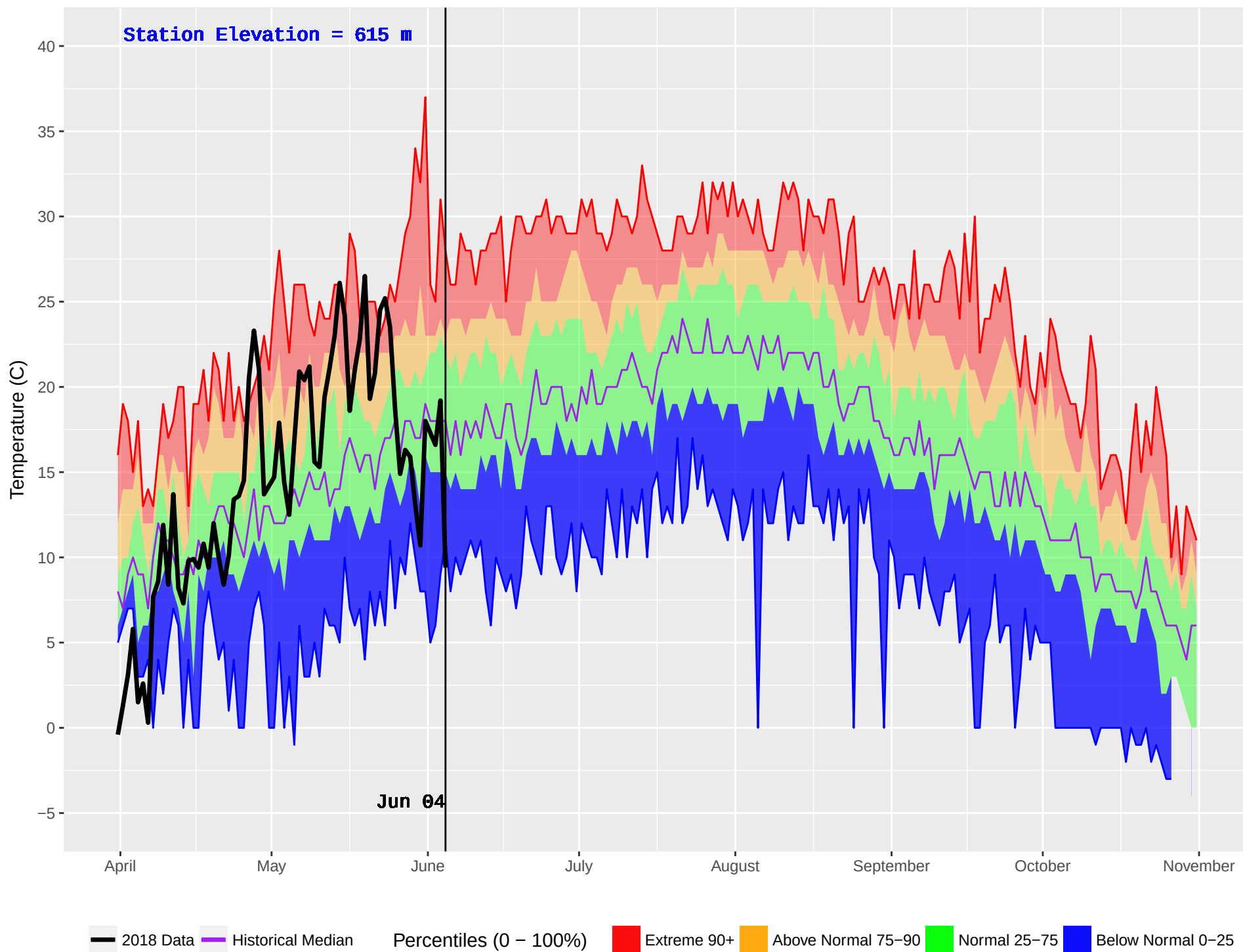
HIXON (187) : Historical (1976–2016) and Current (2018) Noon Temperature
