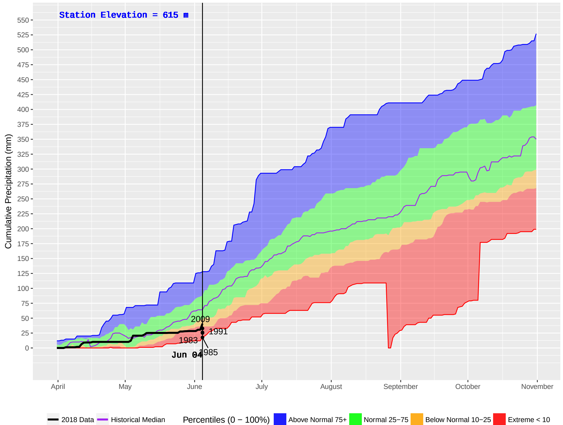
HIXON (187) : Historical (1976–2016) and Current (2018) Noon Cumulative Precipitation
