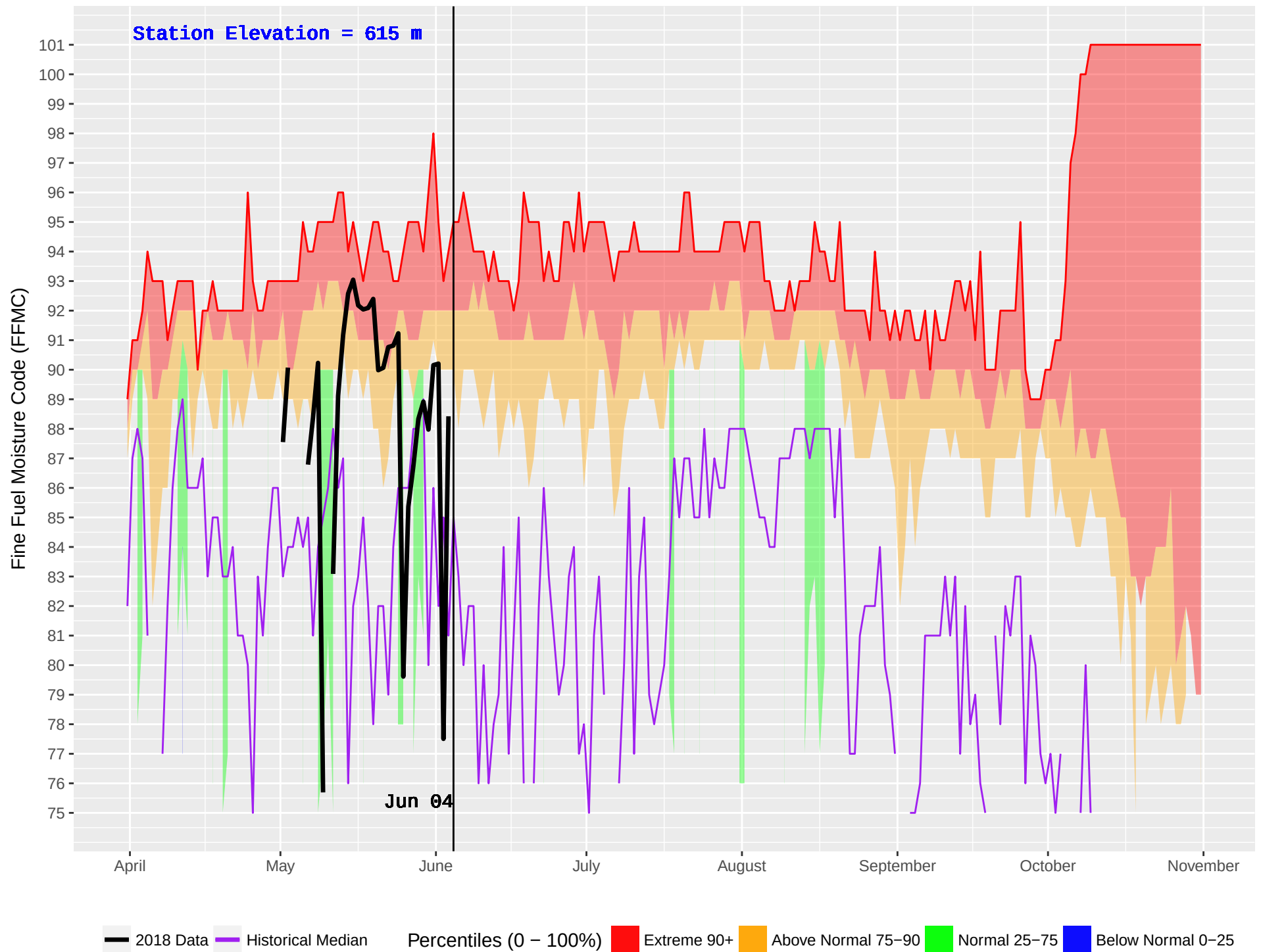
HIXON (187) : Historical (1976–2016) and Current (2018) Noon Fine Fuel Moisture Code (FFMC)
