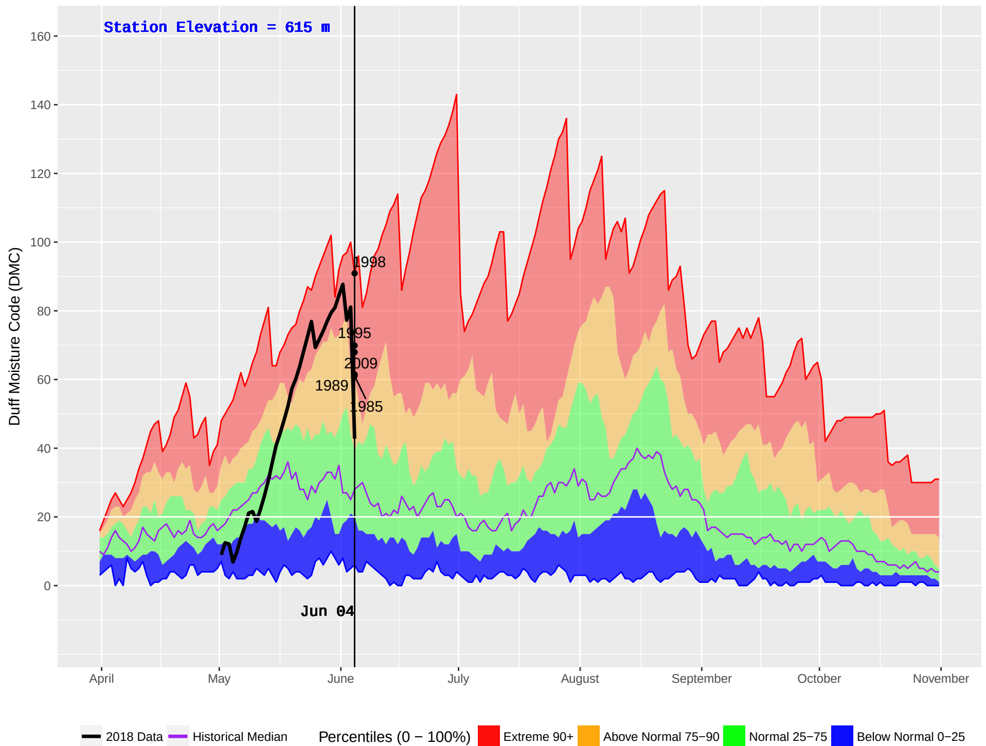
HIXON (187) : Historical (1976–2016) and Current (2018) Noon Duff Moisture Code (DMC)
