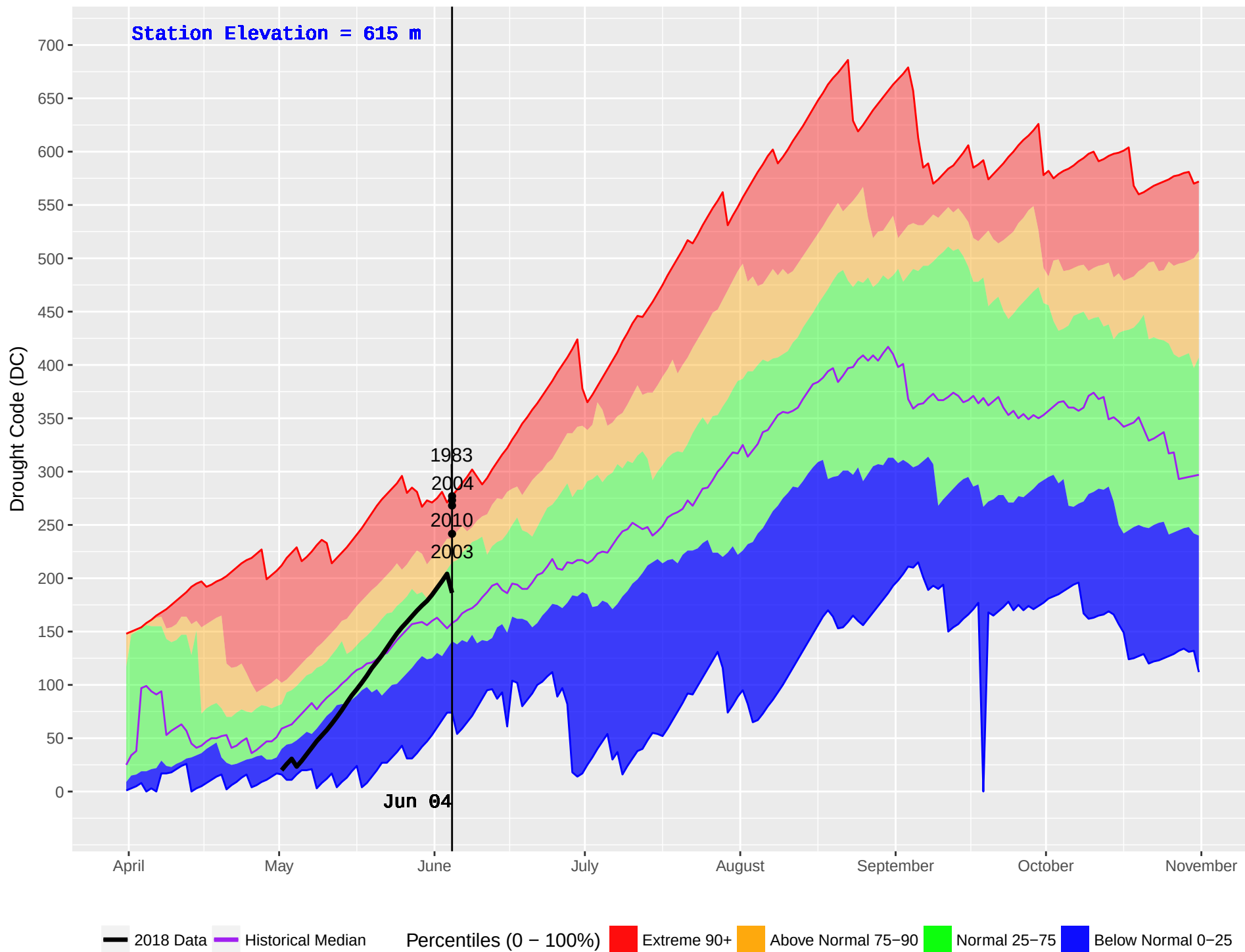
HIXON (187) : Historical (1976–2016) and Current (2018) Noon Drought Code (DC)
